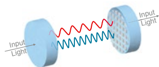
Schematic of an optical cavity resonant for two different wavelengths. The resonance for both wavelengths is achieved by employing dispersion engineered metasurface mirrors.
