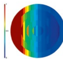
Portion of dendritic ice after stage-one freezing.
