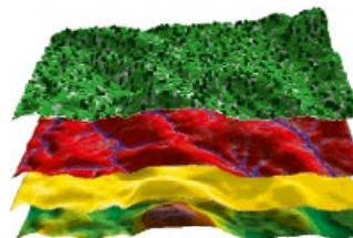
Set of environmental predictors controlling species distribution patterns (top)
