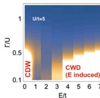
Non-equilibrium phases of matter (blue denotes a metal, white a charge density wave) in an open 1d system with interactions U , reservoirs couplings \Gamma , and an electrical field E .
