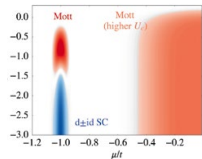
Theoretical prediction for the phase diagram of twisted bilayer graphene as a function of the temperature T and the chemical potential \mu . The system features unconventional superconductivity (SC).
