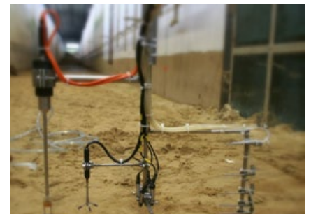
Instrument frame for measurements of sediment transport
