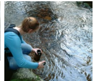
Studies on the release of heavy metal by dissolved organic matter from peatlands (Harz, Germany).
