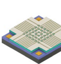
GaN microLED arrays for Structured Micro Illumination Light Engines (SMILE ©) from ec2. Photo: © Jan Gülink, TUBS
