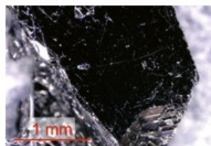
Majorana fermions found in \text{RuCl}_3 have implications for topologically stable systems and quantum computing, Wulferding, D., et al., Nature Communication , (2020).
