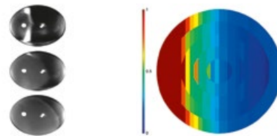
Dendritic freezing of a supercooled water droplet.
