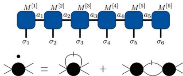
Fundamental building blocks of tensor networks (matrix product states) as well as of the functional renormalization group (flow equations for vertex functions).
