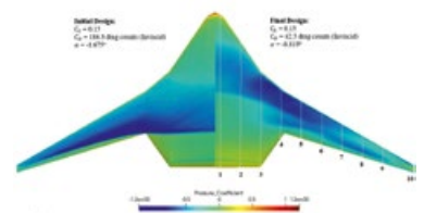
Aircraft aerodynamic shape optimization
