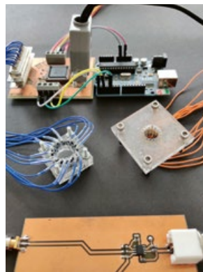
Miniaturized electrical impedance tomographers
