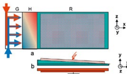
Figure: Schematic of an atmospheric-pressure plasma reactor employing orthogonal gradients of gas composition and power density
