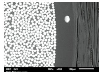
Glass-fiber (GF) rod reinforced wood. The rod is oriented perpendicular to wood fibers. From left to right: white circles = GF fibers, gray = epoxy resin, gray with black spots and marks = wood. ©B. Kasal
