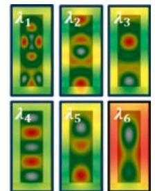
Magnetic field distribution in a multi-resonant metasurface at different resonance wavelengths. Red and white colors respectively indicate field maxima and minima.
