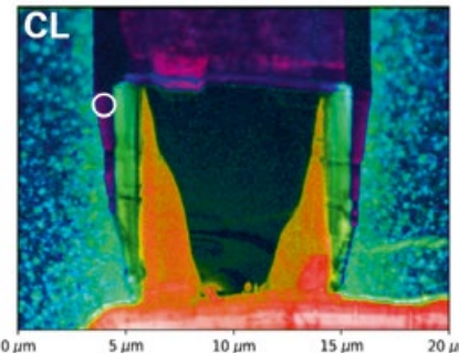
Nanoanalytics of a UV emitting LED structure by spatially resolved e-beam luminescence in LENA. © Christoph Margenfeld, TUBS
