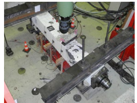
Thin-walled, hollow UHPC-Beam after testing
